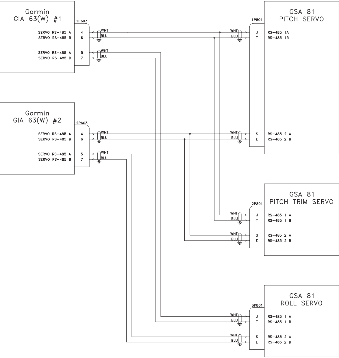
Figure C-1. GIA 63(W) Example Interconnect (Sheet 6 of 7)
