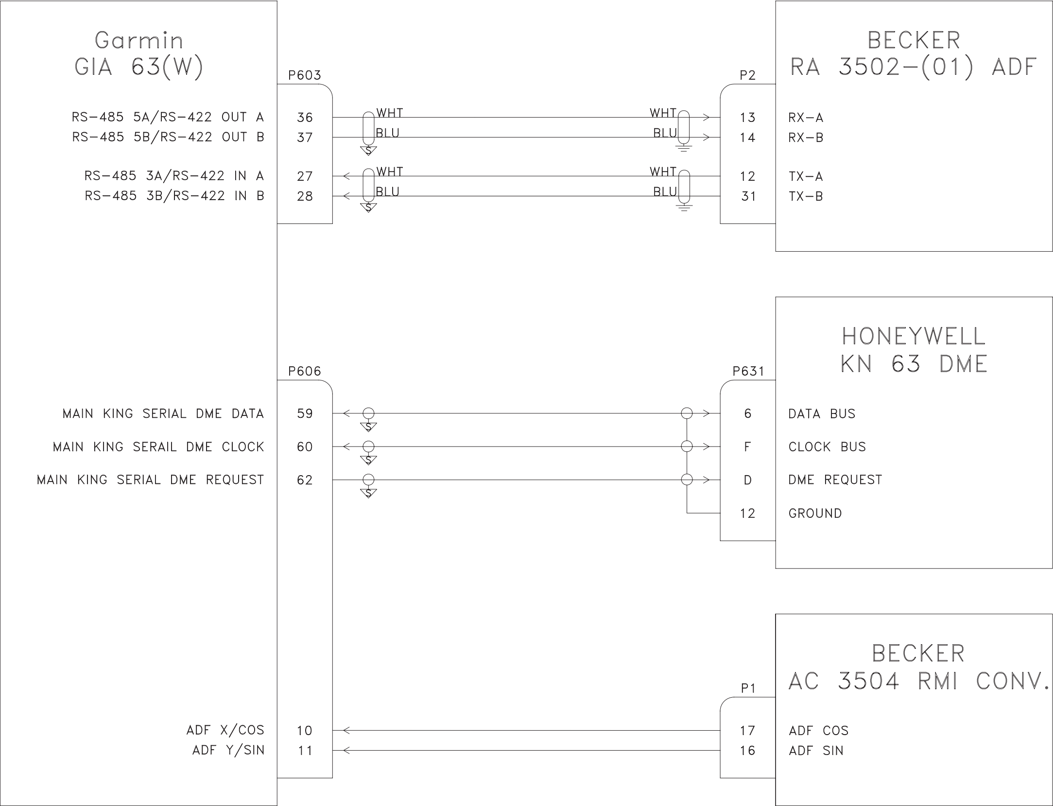
Figure C-1. GIA 63(W) Example Interconnect (Sheet 4 of 7)
