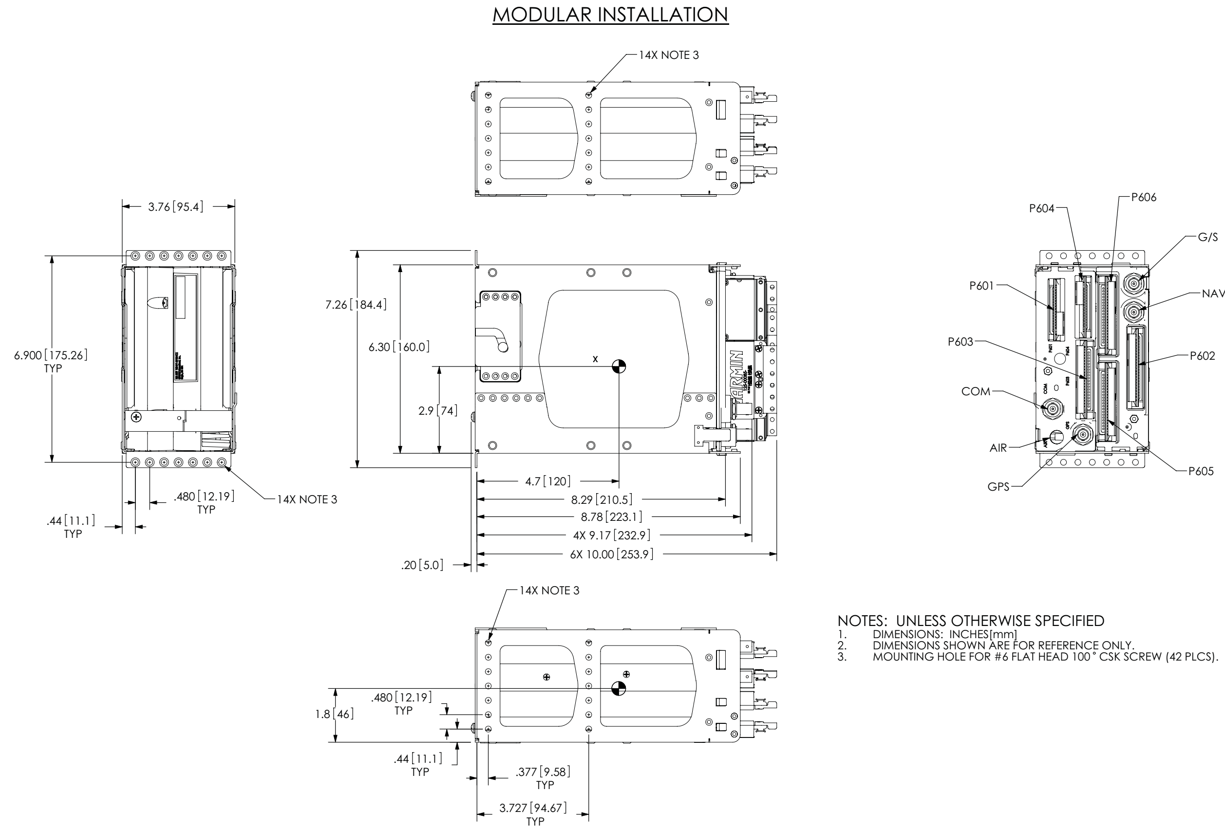
Figure B-1. GIA 63(W) Modular Installation Outline Drawing
