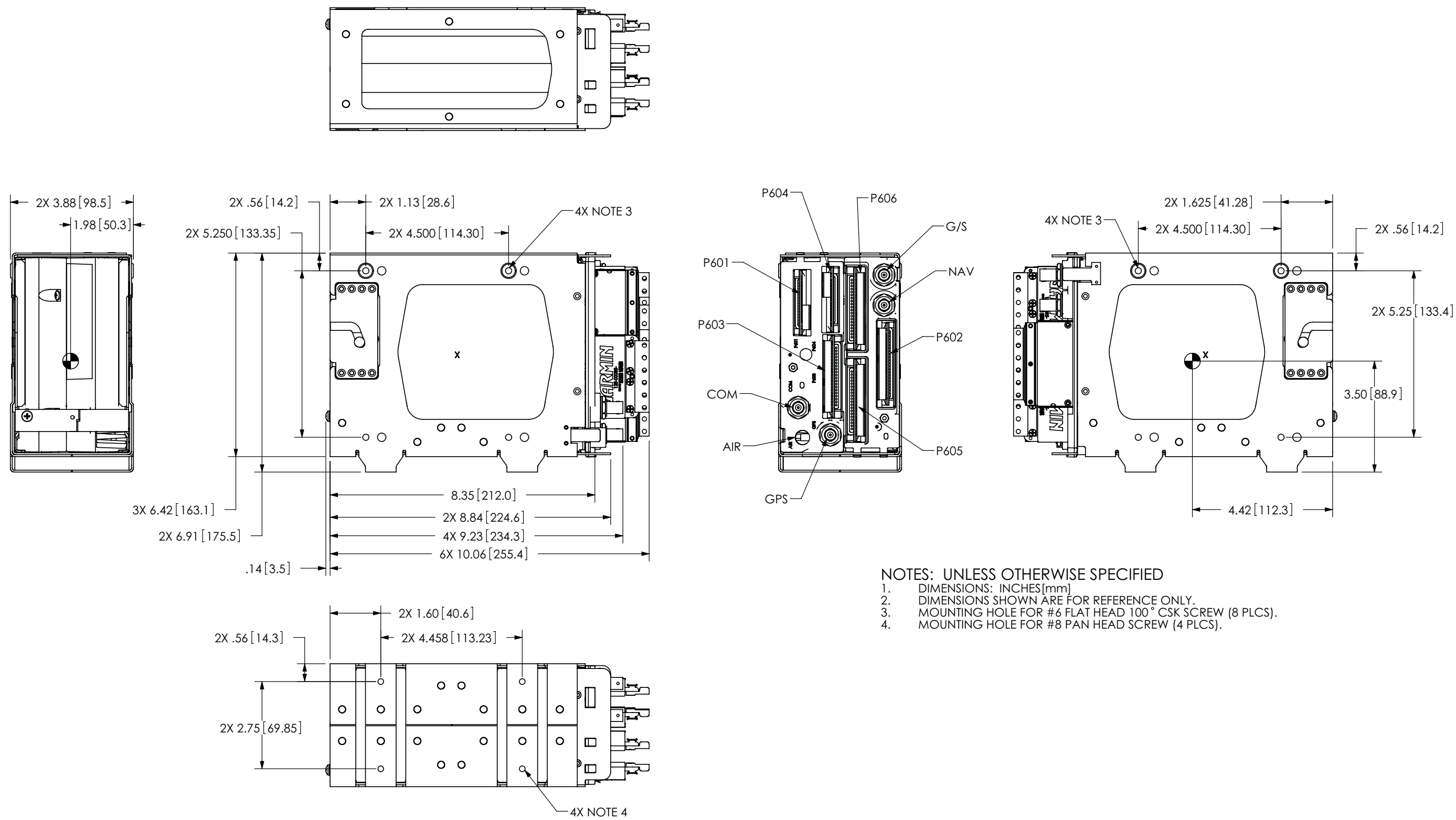
Figure B-3. GIA 63(W) Standalone Installation Outline Drawing
