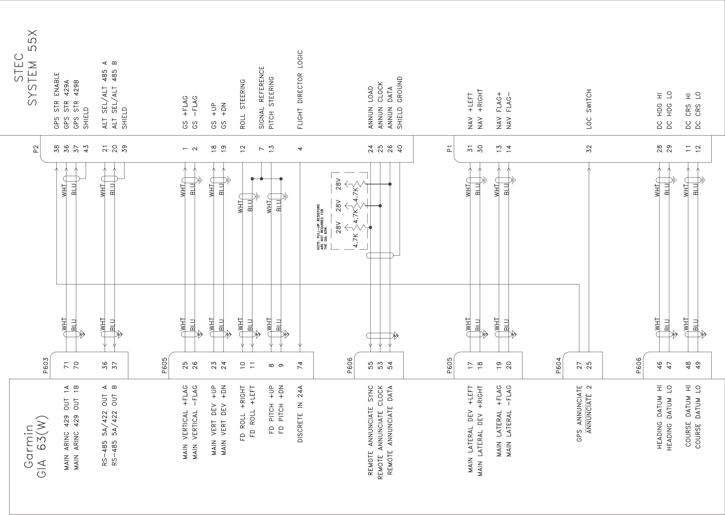
Figure C-1. GIA 63(W) Example Interconnect (Sheet 5 of 7)
